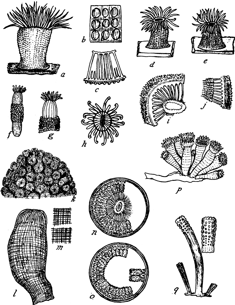
FIGURE 3.— a-c , Cladactella manni Verrill: a , expanded showing surface covered by verrucae (natural size), b , enlarged area of surface of body wall showing linear arrangement of verrucae, c , cross section of wall and mesenteries ( \times 2 ); d-e , Cladactella obscura Verrill, two specimens in expanded condition (natural size); f-h , Edwardsiella carneola Verrill: f , entire specimen expanded, showing coating of foreign material ( \times 2 ), g , distal half of the same specimen ( \times 4 ); h , oral view of same specimen ( \times 8 ); i-j , Zoanthus vestitus : i , transverse section through region of gullet ( \times 8 ), j , transverse section below gullet, showing mesenteries bearing gonads; k-o , Zoanthus confertus : k , colony of contracted polyps (slightly enlarged), l , contracted polyp ( \times 4 ), m , two small areas of body surface ( \times 4 ), n , o , transverse sections of polyp showing numerous mesenteries bearing gonods ( \times 5 ); p , Zoanthus nitidus Verrill, a group of expanded polyps attached to a stolon ( \times 2 ); q , Isaurus elongatus , three partially expanded polyps, young and old with distal portion of one more enlarged from one-half to natural size.
